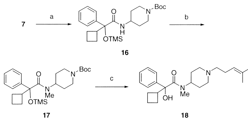
Scheme 3. Conditions: (a) TMSCl, imidazole, DMF; (b) NaH, MeI, n -Bu 4 NI, THF; (c) HCl-MeOH then 10 , K 2 CO 3 , KI, DMF.
