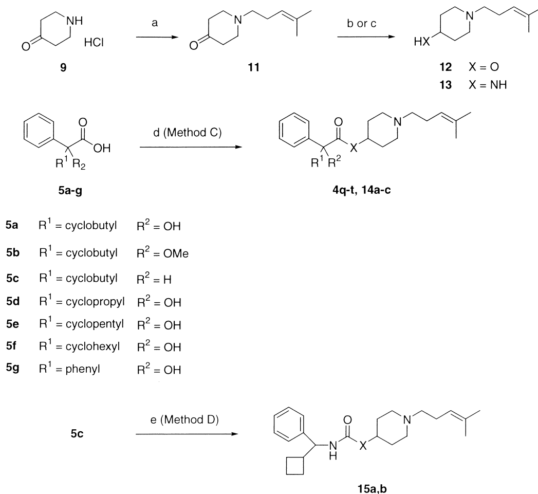
Scheme 2. Conditions: (a) 5-bromo-2-methyl-2-pentene 10 , K 2 CO 3 , KI, DMF; (b) NaBH 4 , MeOH; (c) AcONH 4 , NaBCNH 3 , MeOH; (d) 12 or 13 , WSC-HCl, HOBT; (e) DPPA, toluene then 12 or 13 .
